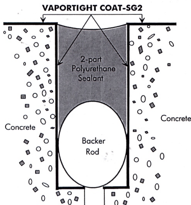
Schematic sketch
