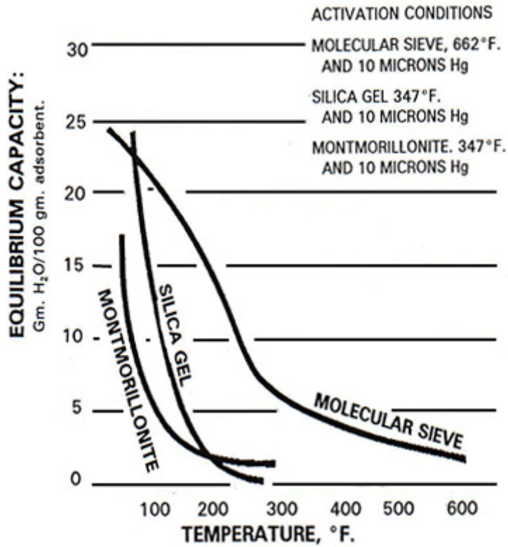
Figure 1: Equilibrium H 2 O capacity. (P H 2 O = 0.407 in. Hg)
