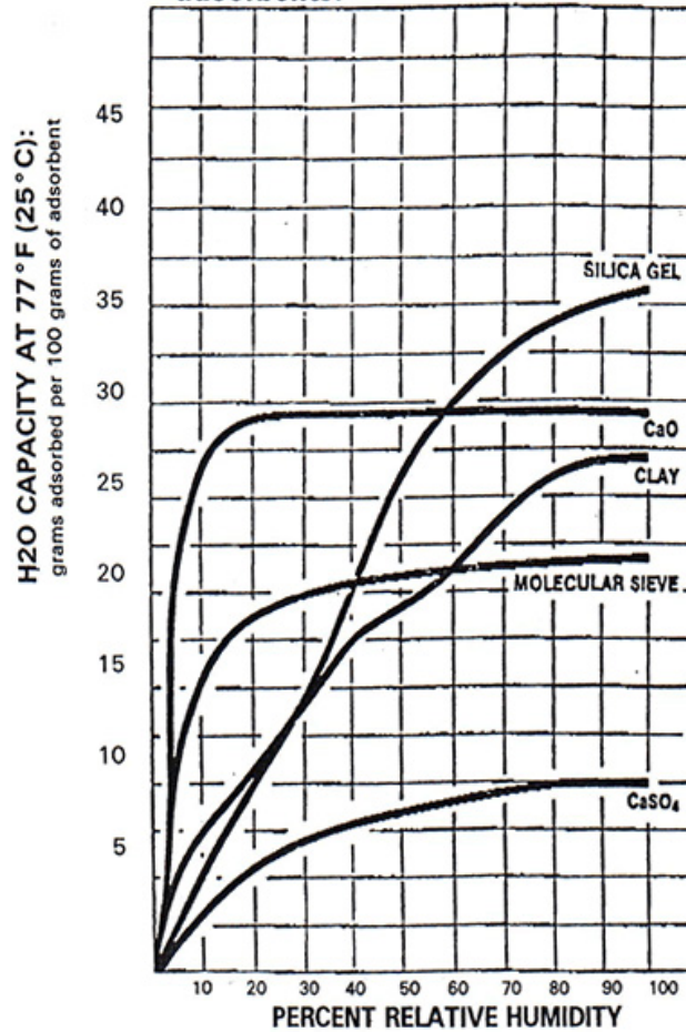
Figure 2: Equilibrium capacity (H 2 O) of various adsorbents.
