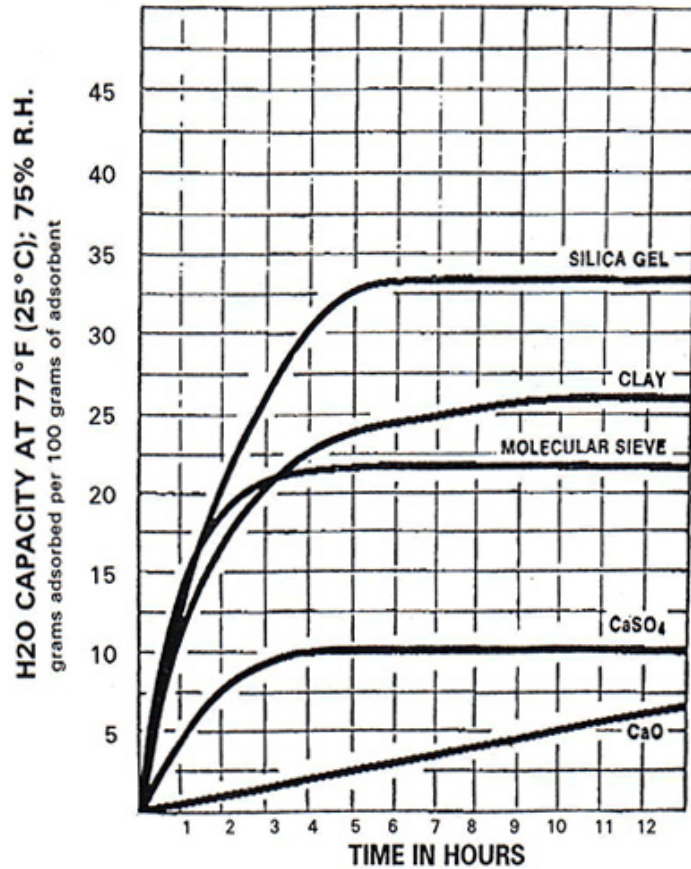
Figure 3: Adsorption rate(H 2 O) of various adsorbents.
